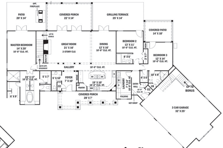
main floor
